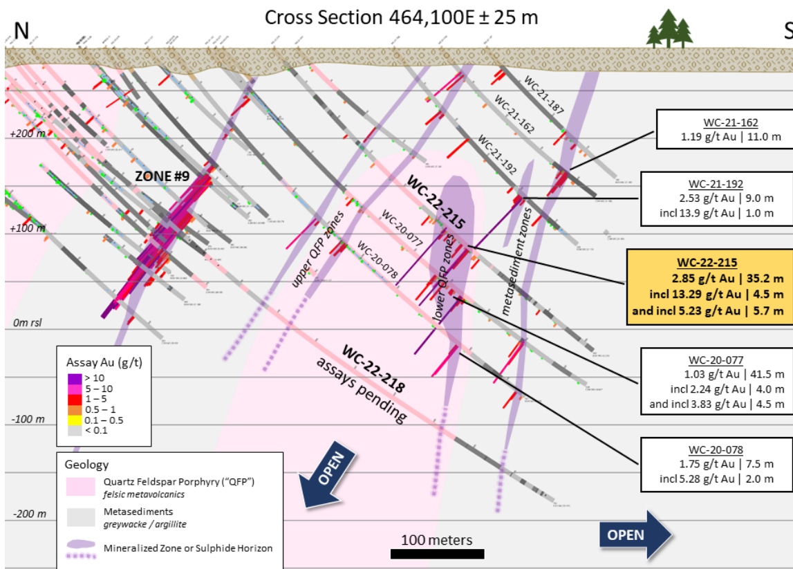
Figure 1 – Cross Section 464,100E with recent 2022 drillholes
